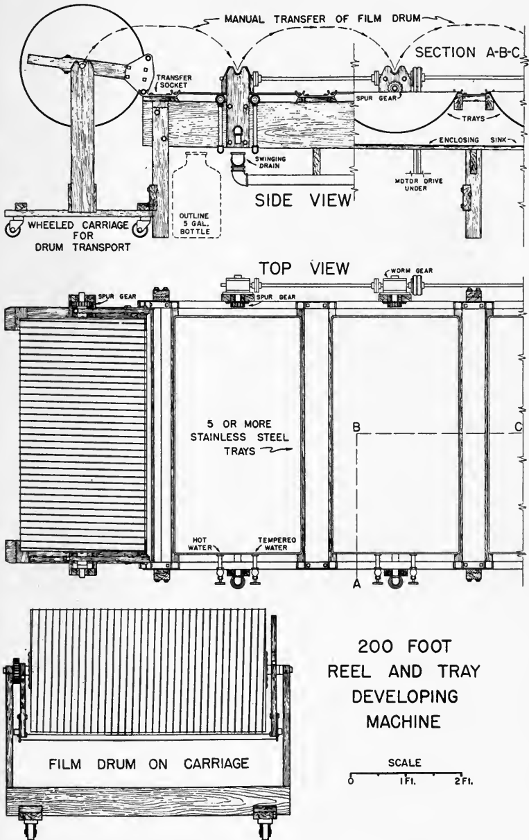
FIG. 3. Two-hundred ft reel and tray developing machine.
